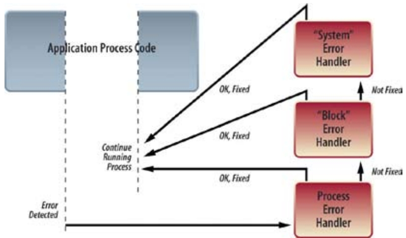
Figure 13. Enea OSE Error Escalation Sequence.
