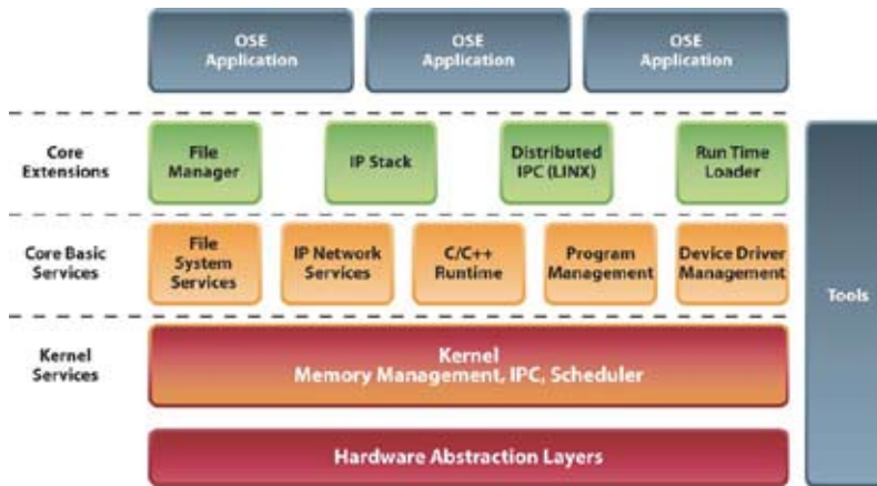
Figure 2. OSE's Modular, Layered Architecture.
