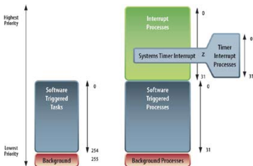
Figure 4. Typical RTOS Priority Schema (left) vs. Enea OSE Priority Process (right).
